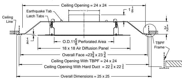
Models: 5750-T-1 ( Steel - Surface Mount - 24 x 24 ) 5750-T-1 AS ( Aluminized Steel - Surface Mount - 24 x 24 ) 5750-T-1 AL ( Aluminum - Surface Mount - 24 x 24 )
