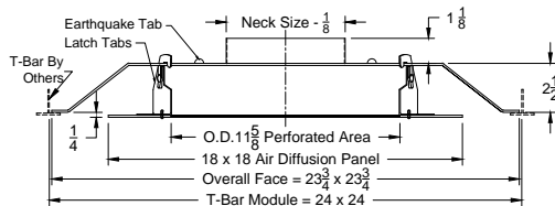
Models: 5750-T-9 ( Steel - Bolt Slot / Donn Finline Grid ) 5750-T-9 AS ( Aluminized Steel - Bolt Slot / Donn Finline Grid ) 5750-T-9 AL ( Aluminum - Bolt Slot / Donn Finline Grid )
