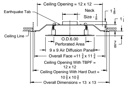
Models: 5750-T-6 ( Steel - Lay In T-Bar - 12 x 12 ) 5750-T-6 AS ( Aluminized Steel - Lay In T-Bar - 12 x 12 ) 5750-T-6 AL ( Aluminum - Lay In T-Bar - 12 x 12 )
