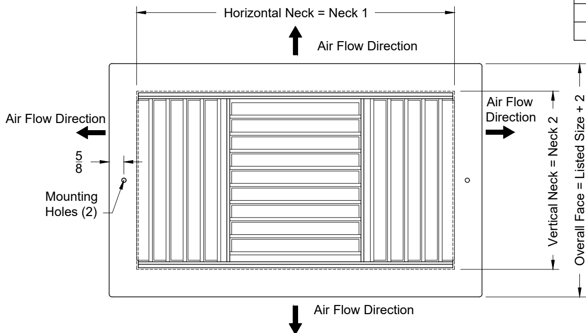
Face View
