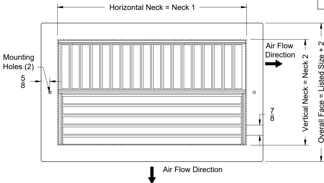
Face View
