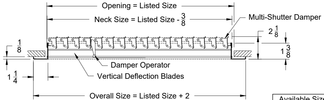
Side View
