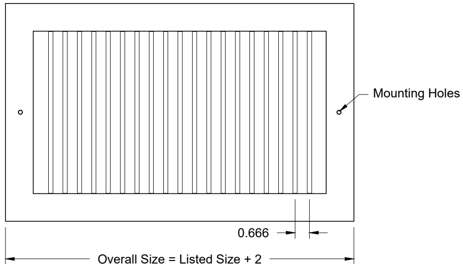
Face View
